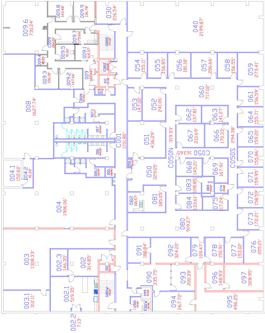
Washington Court Place BASEMENT PLAN BUILDING #031 26703.56 SQUARE FEET
